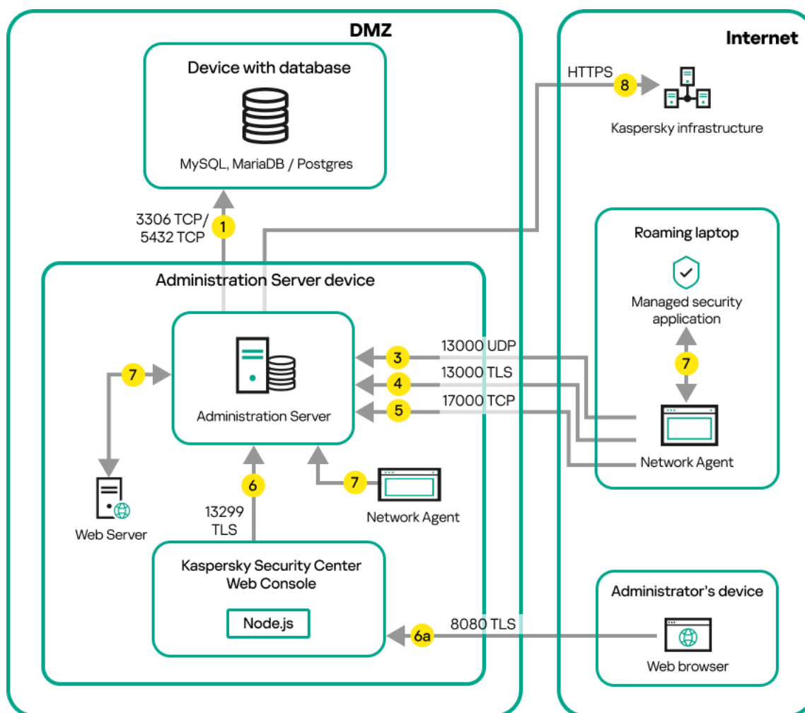
Administration Server in DMZ, managed mobile devices on the internet
